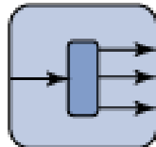
Event propagation
