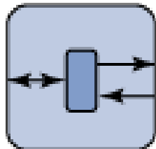
Request / response
